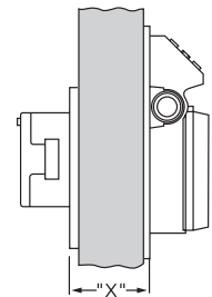
"X" = Container Thickness for Lock Mounting Purposes
